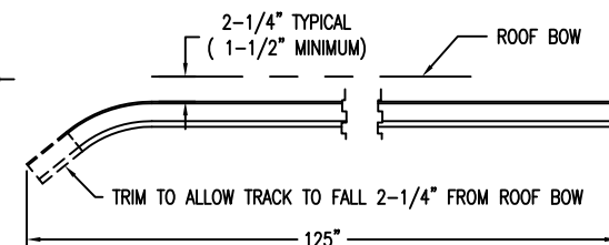
VERTICAL TRACK DETAIL
