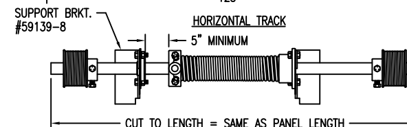
COUNTERBALANCE ASSEMBLY
