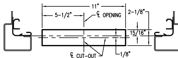
DETAIL OF CUT-OUT IN SILL FOR 70093 LOCK CATCH BOX
