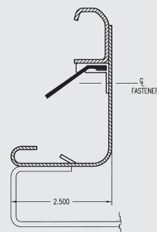
End Seal Assembly
