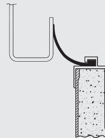
Panel Mounted – Rubber Seal Retainer – #70083 Seal – # 69718
