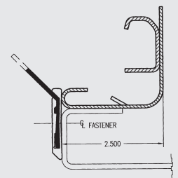
Secondary Seal Assembly
