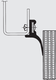
Header Mounted – Rubber
