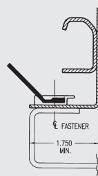
Seal Assembly Belted Material #69922 (Long Lip #70362)
