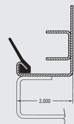
Side Seal #39235
